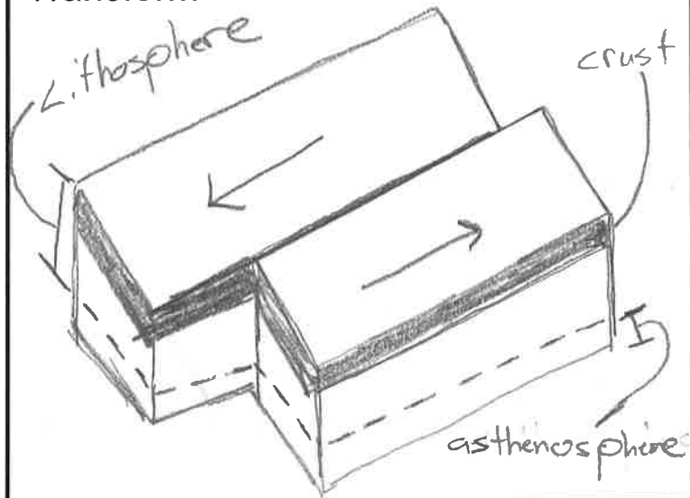
Transform
